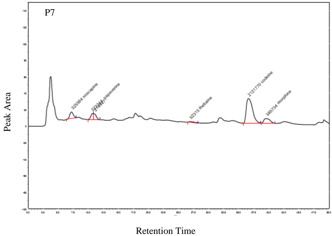
Supplementary Figure 1. HPLC chromatograms of major alkaloids (morphine, codeine, thebaine, noscapine, and papaverine) in seven populations (P1-P7) of opium poppy ( Papaver somniferum L.) from Afghanistan.
