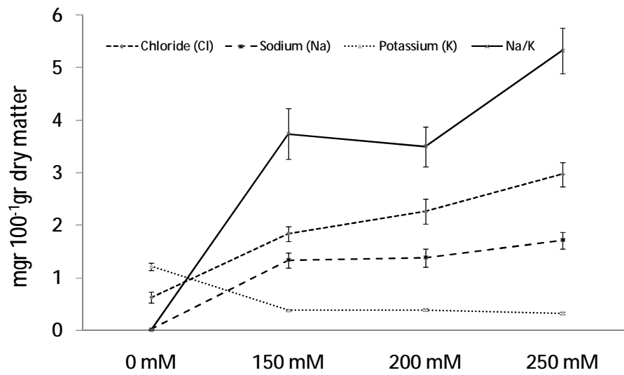
Figure 2. Changes in ionic concentration of Cl - , Na + , K + and Na + / K + ratio averaged over all wheat genotypes.
