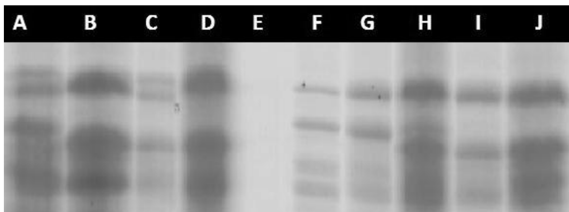
Figure 4. SDS-PAGE banding patterns of Glu-1D loci in the wheat genotypes (from left to right; A: Cajema×Ho2, B: Ho2, C: Cajema×Lerma Roja, D: Lerma Roja, E: No sample (control), F: Chines Spring, G: Cajema×Sette Cerros, H: Cajema, I: Sette Cerros and J: Axona).
