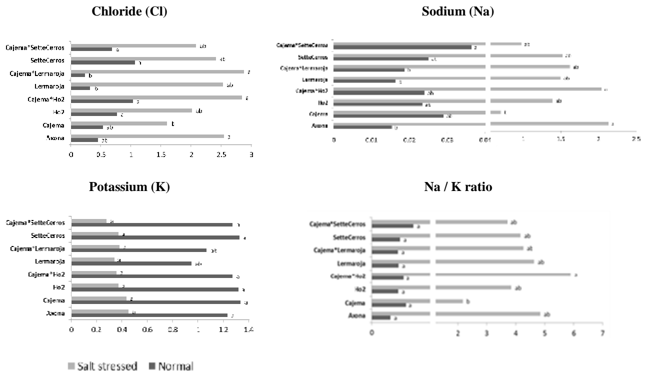
Figure 3. The means of Cl - , Na + and K + concentrations as well as Na + / K + ratio in wheat genotypes. The concentrations are given in mg 100 -1 gr dry matter.
